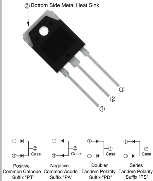
TO-3PN
